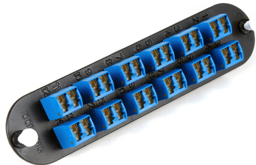
Closet Connector Housing (CCH) Panel, LC adapters, Duplex Shuttered, UPC, 24 F, Single-mode (OS2)
